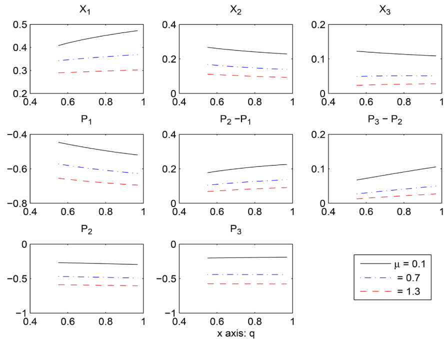
Figure 1. Price dynamics ( D_0 = 0 , Y_0 = 1 , X_0 = 0 , \lambda = 1 , and g = 0 ).
